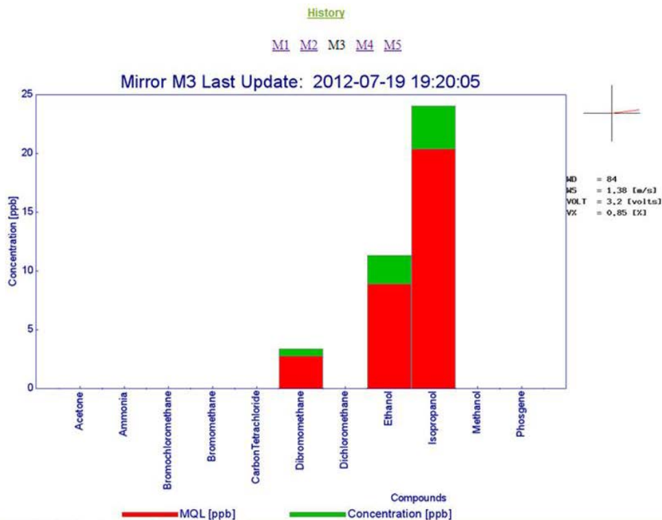
Figure 3. Screenshot of real time OP-FTIR data from a pesticide manufacturing facility (Source: Atmosfir Optics Ltd.)
