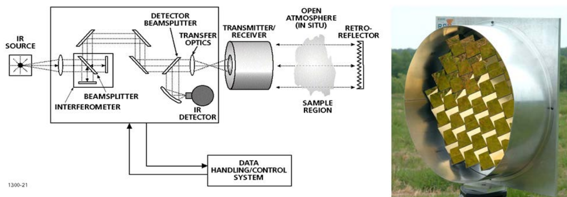
Figure 2. Illustration of an active monostatic OP-FTIR sensor
