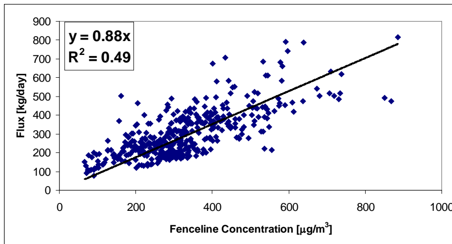
Figure 6. Relationship between Hg mass flux as measured using VRPM and fence-line concentration as measured using a single beam UV-DOAS at a chlor-alkali plant
